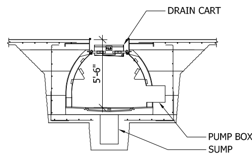
SERVICE BAY SECTION \frac{1}{4}'' = 1'-0'' AT PUMP BOX
