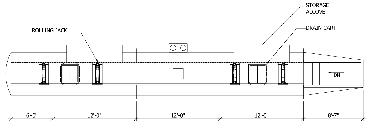
42' IN-LINE STAIR AT RIGHT \frac{1}{4}'' = 1'-0''
