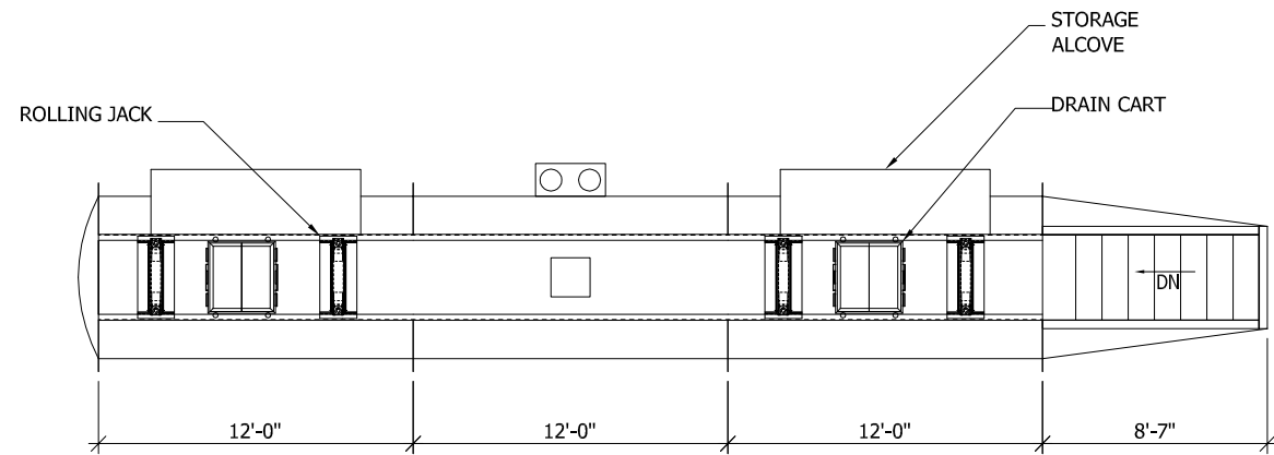
36' IN-LINE STAIR AT RIGHT \frac{1}{4}'' = 1'-0''
