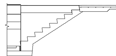
IN-LINE STAIR SECTION \frac{1}{4}'' = 1'-0''
