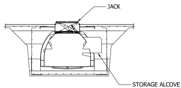
SERVICE BAY SECTION \frac{1}{4}'' = 1'-0'' AT STORAGE ALCOVE
