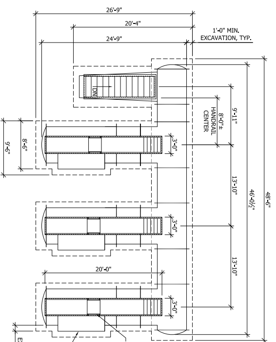
3X20 STAIR SET LEFT (FLAT OR TANK) 1/8"=1'-0"
