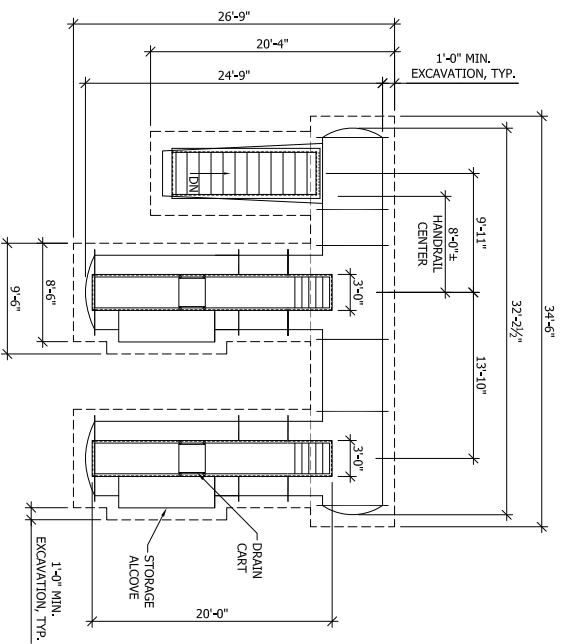
2X20 STAIR SET LEFT (FLAT OR TANK) 1/8"=1'-0"
