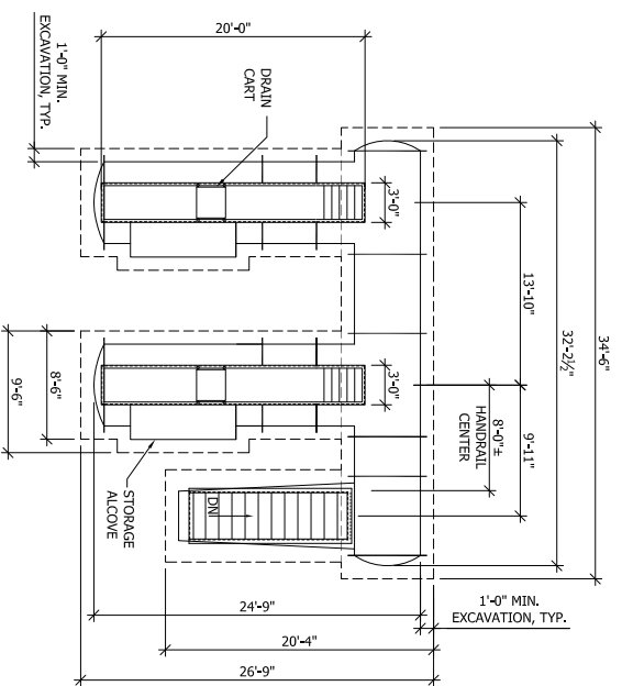
2X20 STAIR SET RIGHT (FLAT OR TANK) 1/8"=1'-0"
